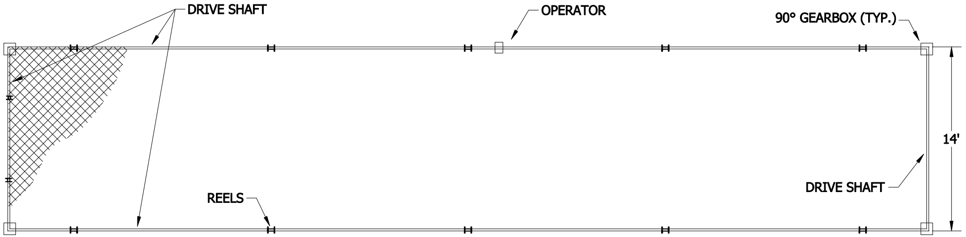
PLAN VIEW
