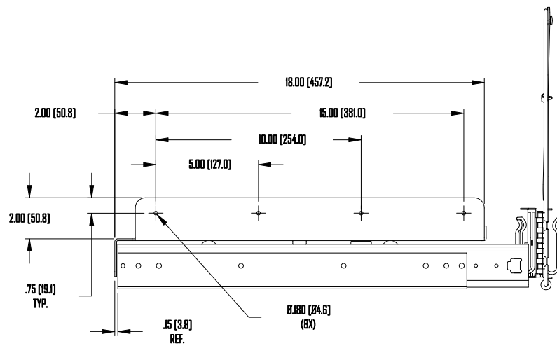
BOTTOM SWIVEL ASSEMBLY, CBMAC-050 WITH ASSEMBLED CABLE CARRIER, CCI-510 ARE SHOWN.
