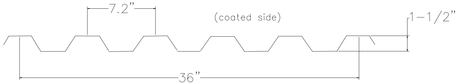
HR-36 (Typical Roof Application)
