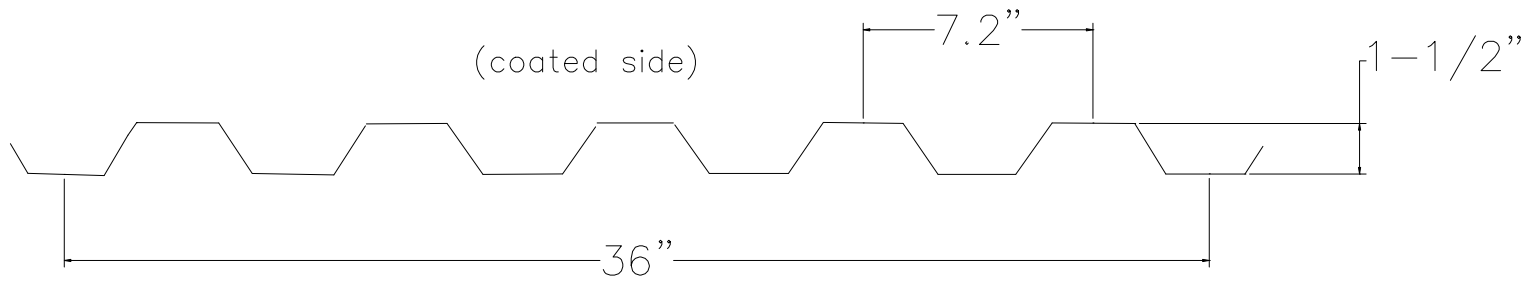
Reversed HR-36 (Typical Wall Application)
