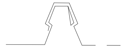
Detail of interlocking rib
