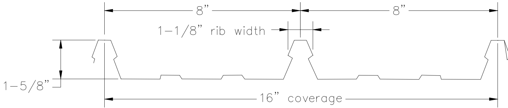
KLIP RIB PROFILE
