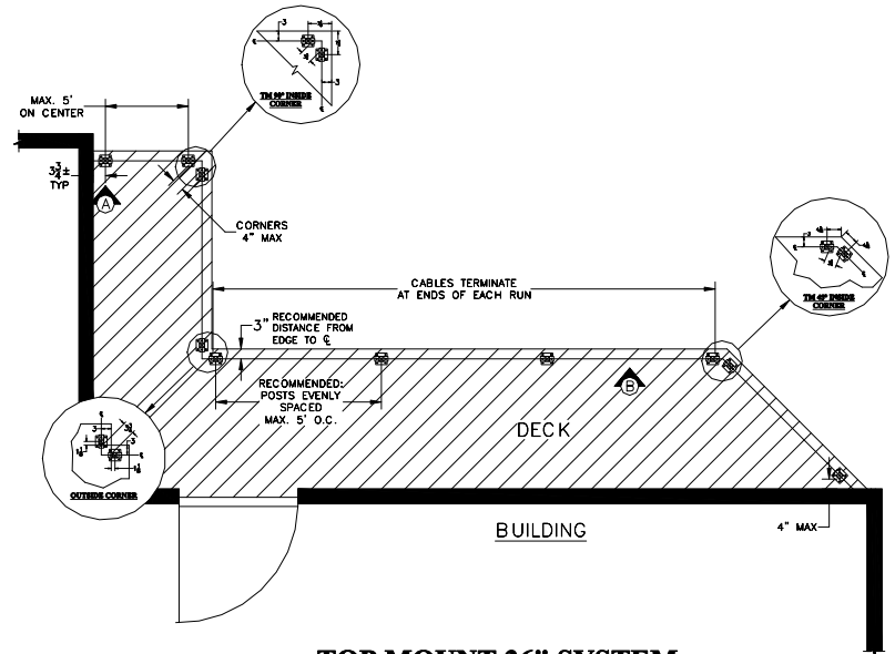
2 TOP MOUNT 36" SYSTEM WITH STOCK MOD FOR WOOD RAIL COMPONENTS CONTACT AGS FOR CUSTOMIZATION OPTIONS 888-842-9492 OR info@agsstainless.com
