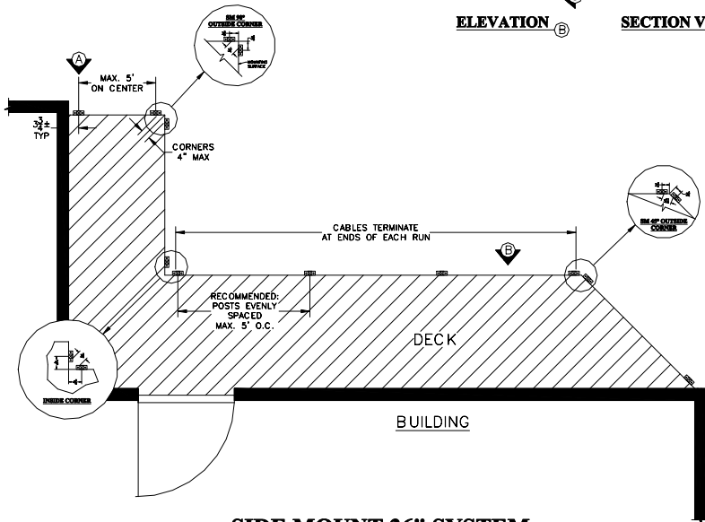
1 SIDE MOUNT 36" SYSTEM WITH STOCK MOD FOR WOOD RAIL COMPONENTS CONTACT AGS FOR CUSTOMIZATION OPTIONS 888-842-9492 OR info@agsstainless.com
