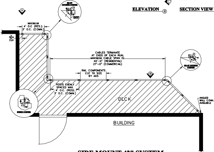
1 SIDE MOUNT 42" SYSTEM WITH STOCK ROUND TOP RAIL COMPONENTS CONTACT AGS FOR CUSTOMIZATION OPTIONS 888-842-9492 OR info@agsstainless.com
