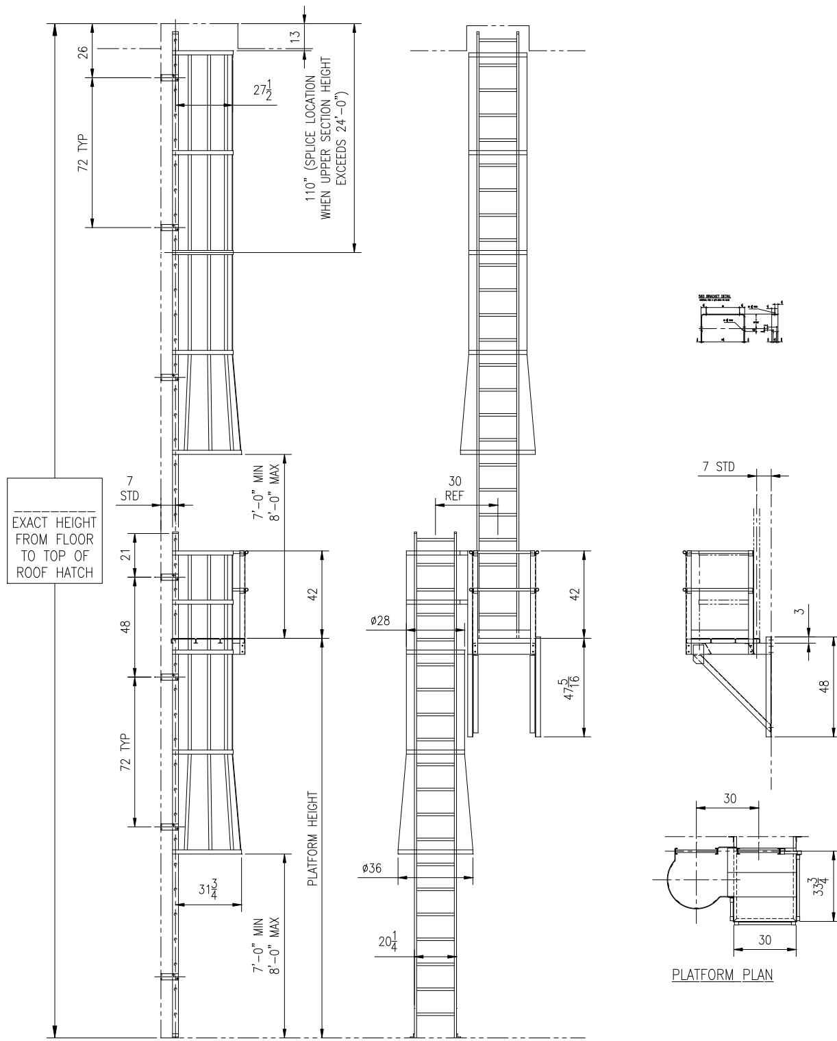
MODEL 560C FIXED WALL LADDER INTERMEDIATE PLATFORM
