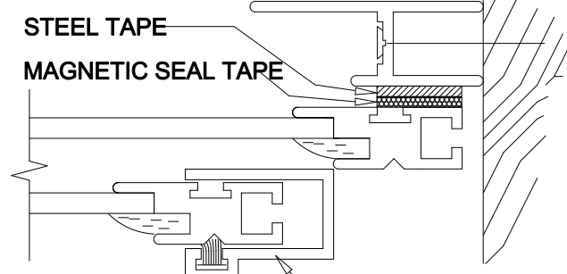
2 JAMB DETAIL SCALE: FULL
