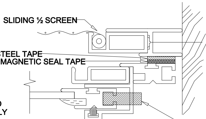
2 JAMB DETAIL SCALE: FULL
