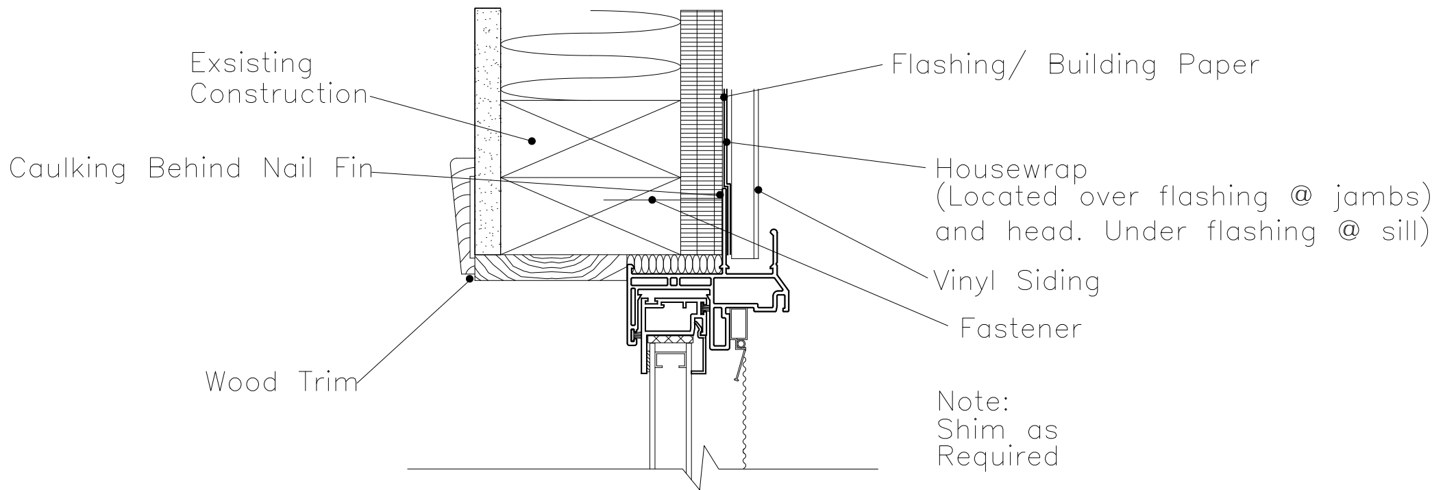
MODEL 0102 JAMB INSTALLATION SCALE: 3"=1'-0" 0740005
