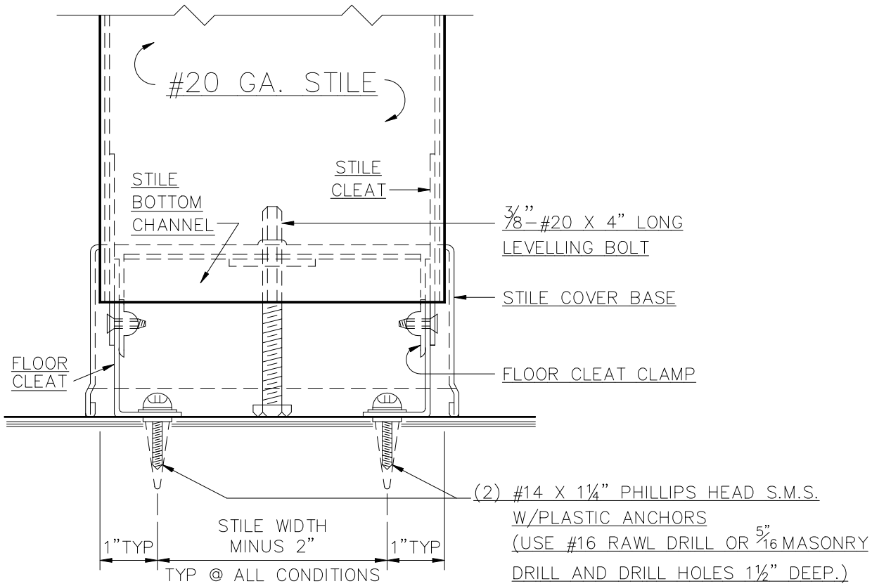
TYPE B.E.-F.F. STILE FASTENING ASSEMBLY
