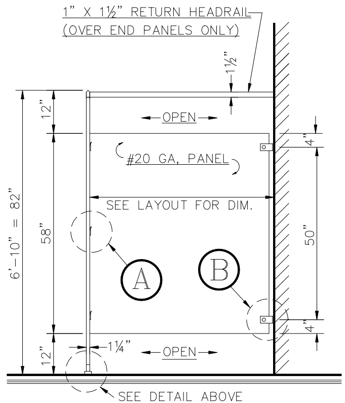
TYPE B.E.-F.F. STILE & PANEL INSTALLATION
