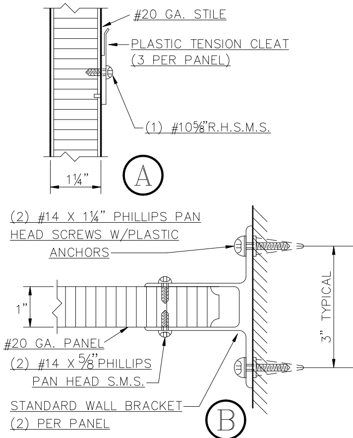
TYPE B.E.-F.F. STILE & PANEL INSTALLATION
