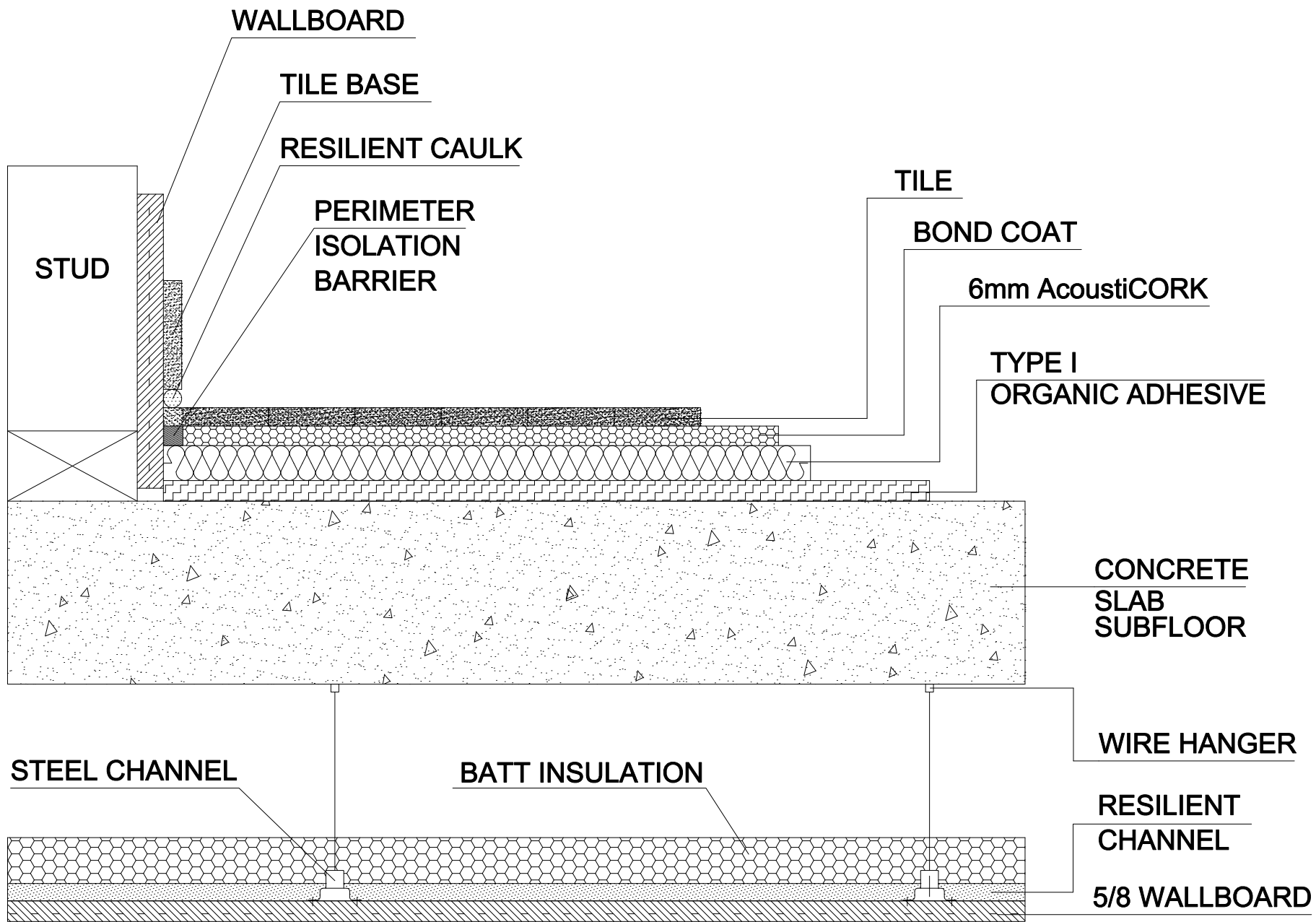
Tile Floors on a 6" Concrete Slab
