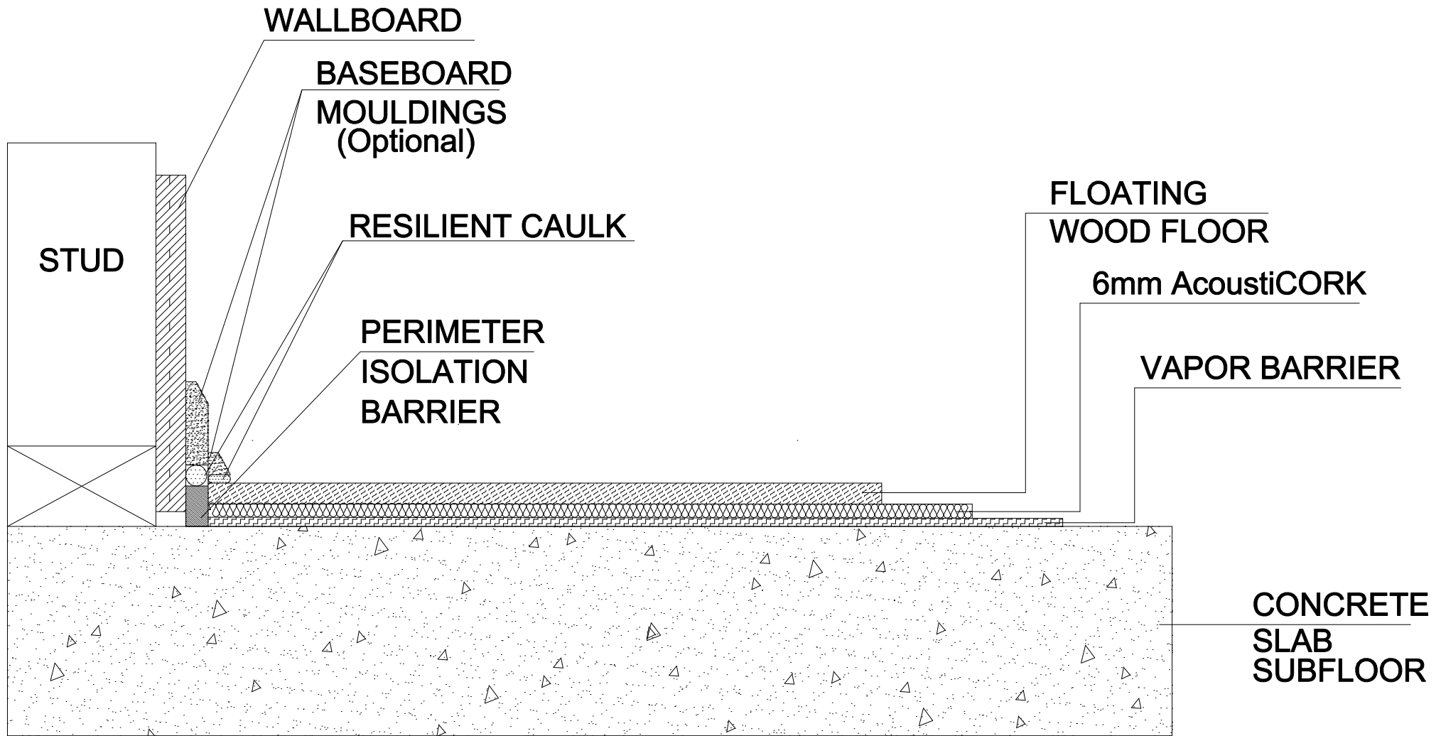
Floating Wood Floors on a Concrete Slab without Suspended Ceiling
