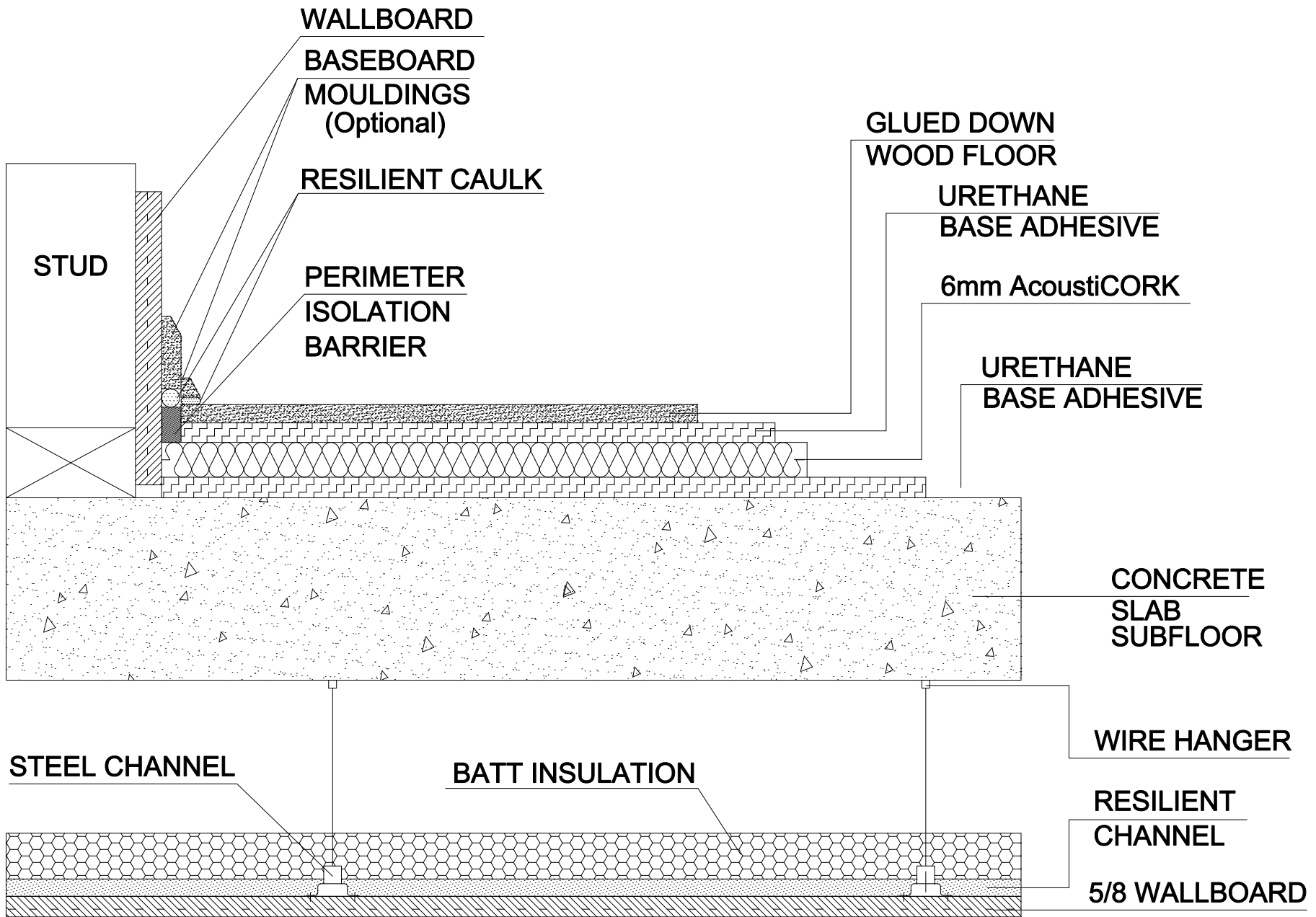
Glued Down Wood Flooring on a Concrete Slab
