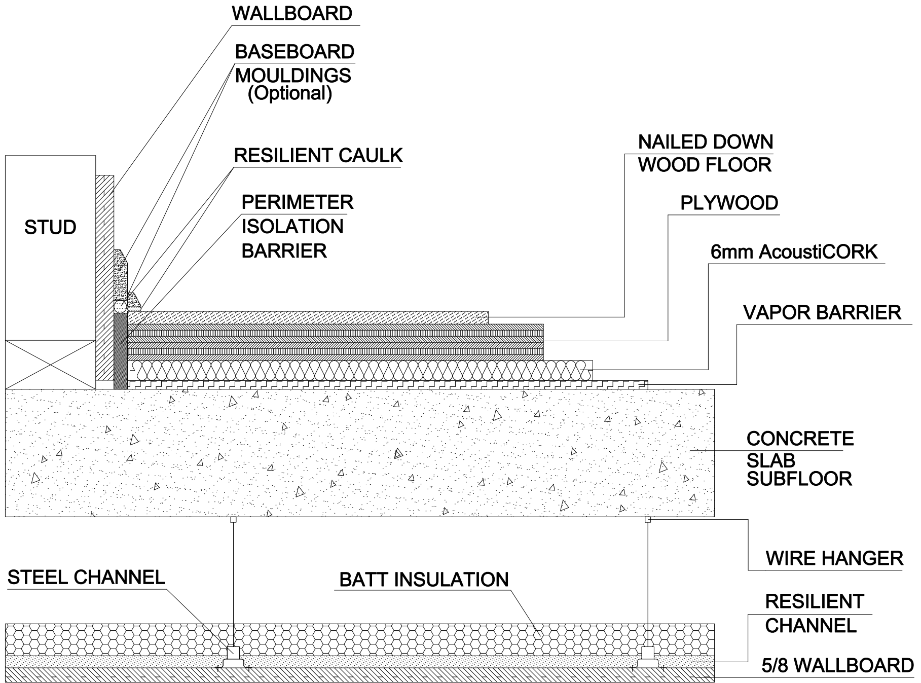
Nailed Down Wood Flopping on a Concrete Slab
