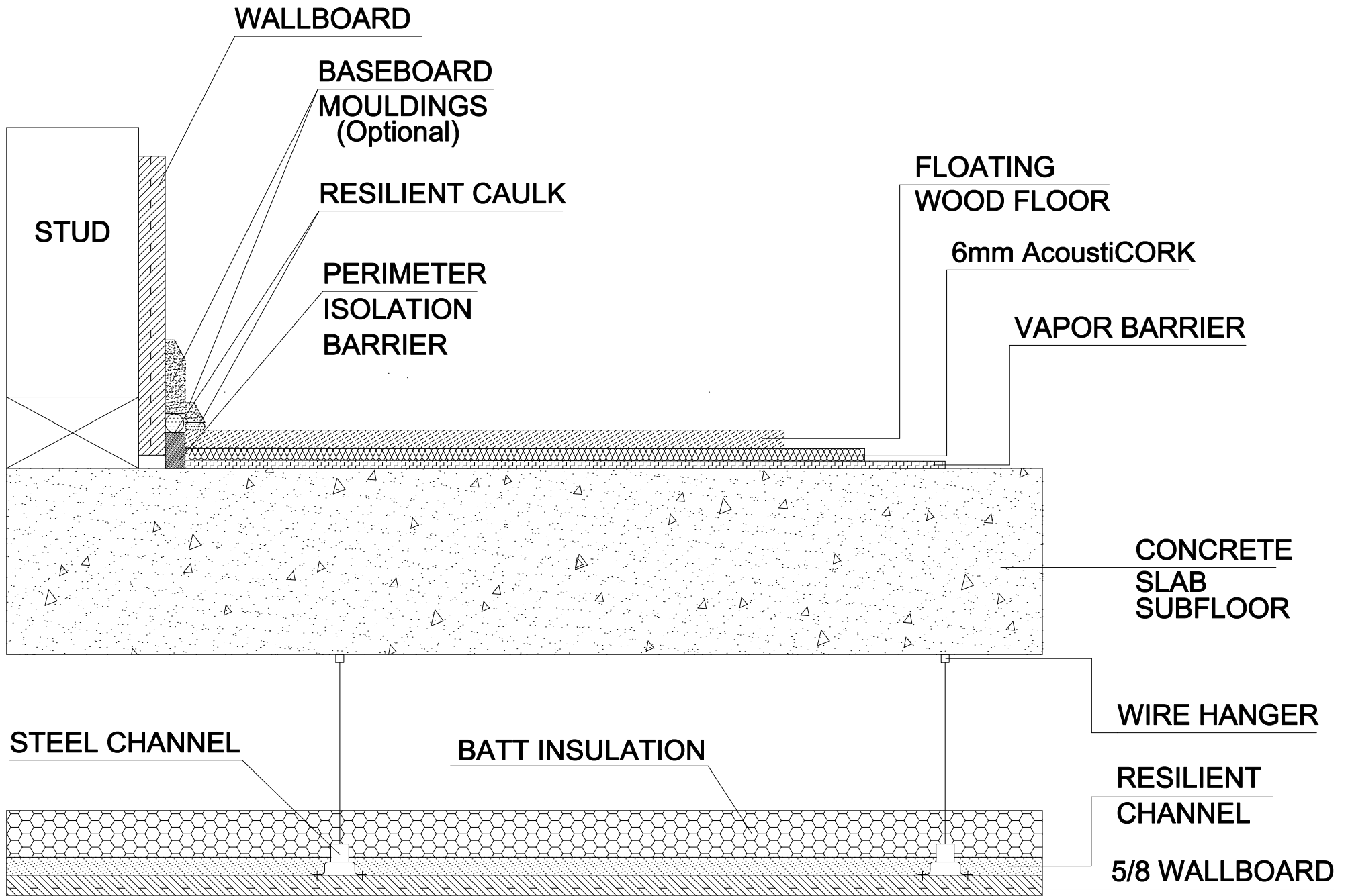
Floating Wood Floors on a Concrete Slab
