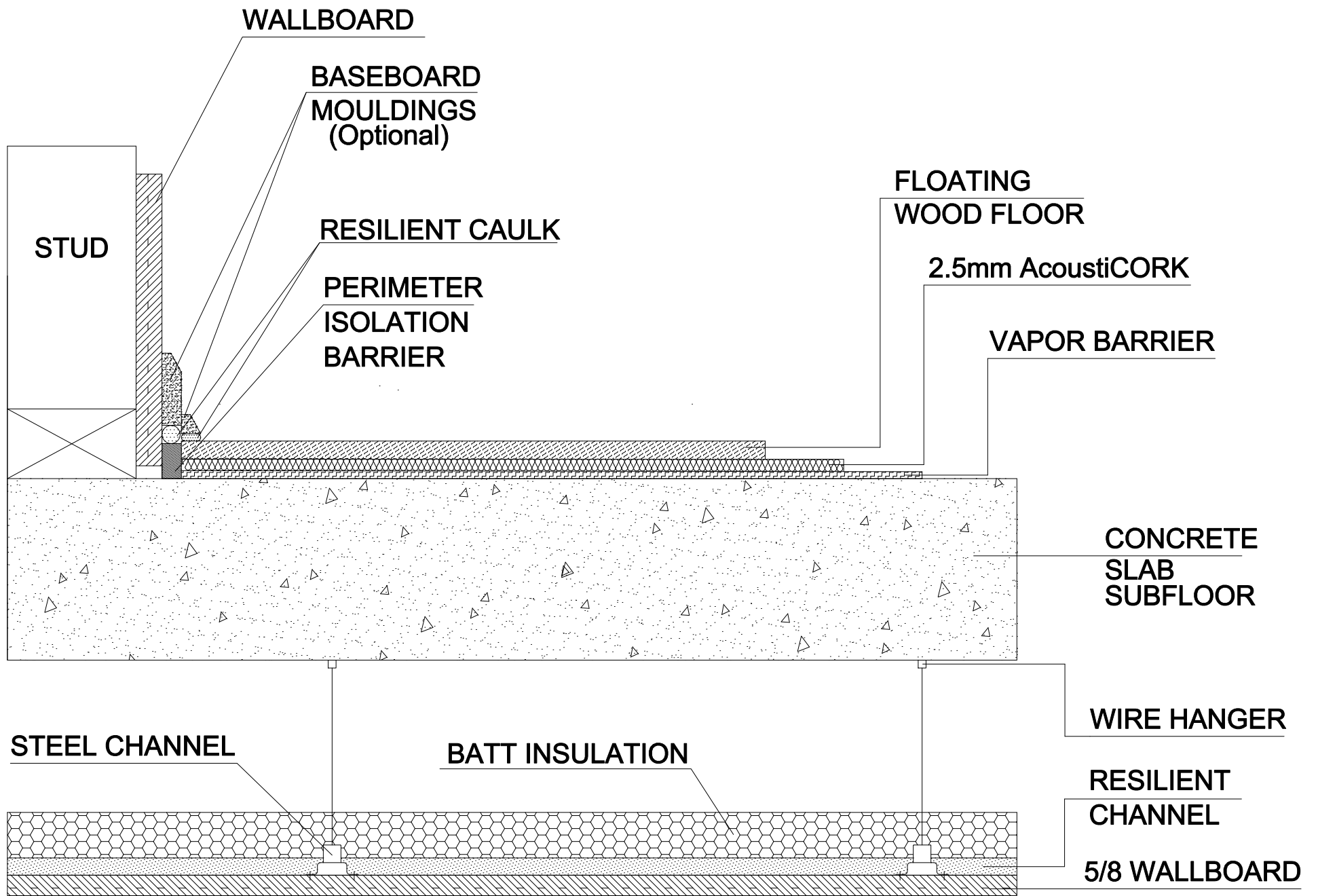
Floating Wood Floors on a Concrete Slab with 2,5mm AcoustiCORCK
