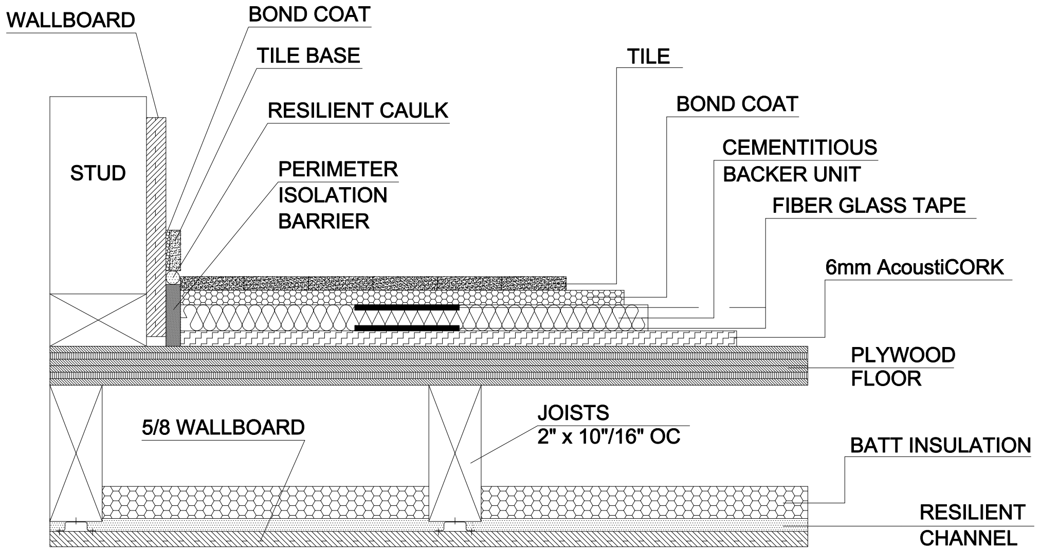
Tile Floors over 1/2" CBU's on a Wood Floor
