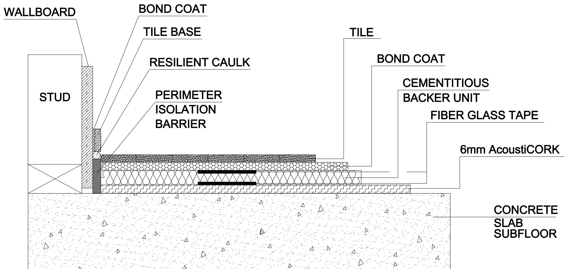
Tile Floors over 1/2" CBU's on a Concrete Slab
