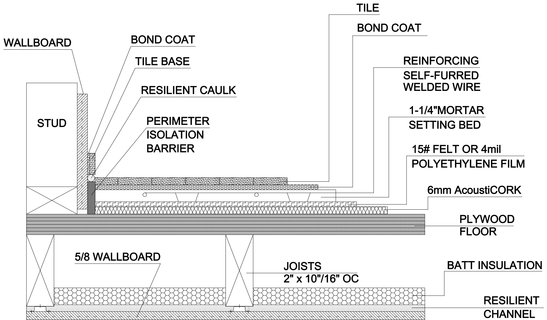
Tile Floors over 1-1/4" Mortar Setting Bed on a Wood Floor
