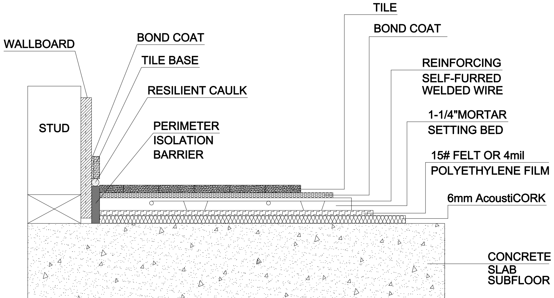
Tile Floors over 1-1/4" Mortar Setting Bed on a Concrete Slab
