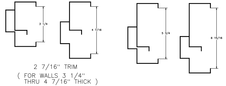
ASSEMBLED FRAME
