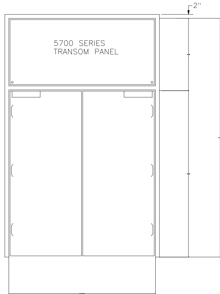
ASSEMBLY UNIT
