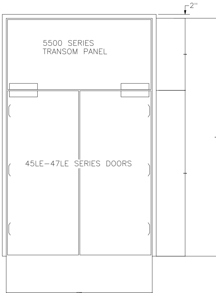
ASSEMBLY UNIT
