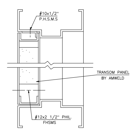
SERIES 5700 TRANSOM OR SIDELIGHT PANEL DETAIL
