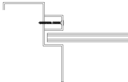
1/4" GLASS DETAIL
