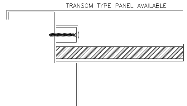
SERIES 400 INSULATED PANEL
