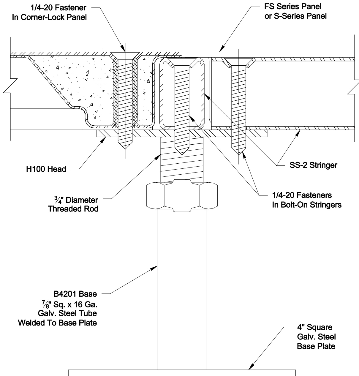
SIDE ELEVATION DETAIL
