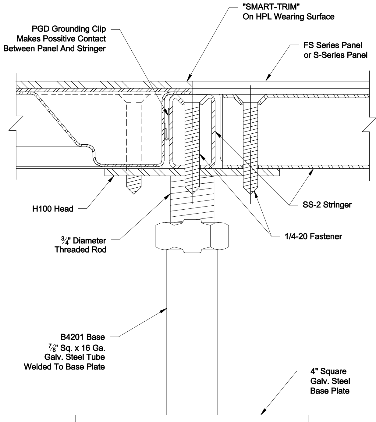
SIDE ELEVATION DETAIL
