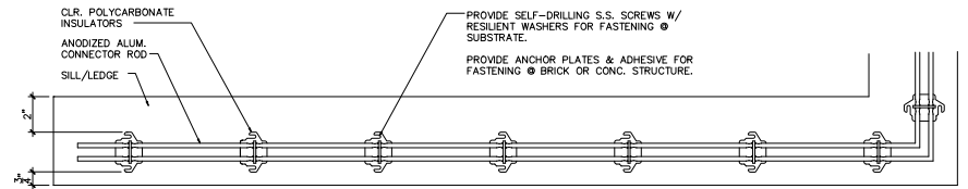
TOP VIEW WITH CORNER ATTACHMENT, TYP.
