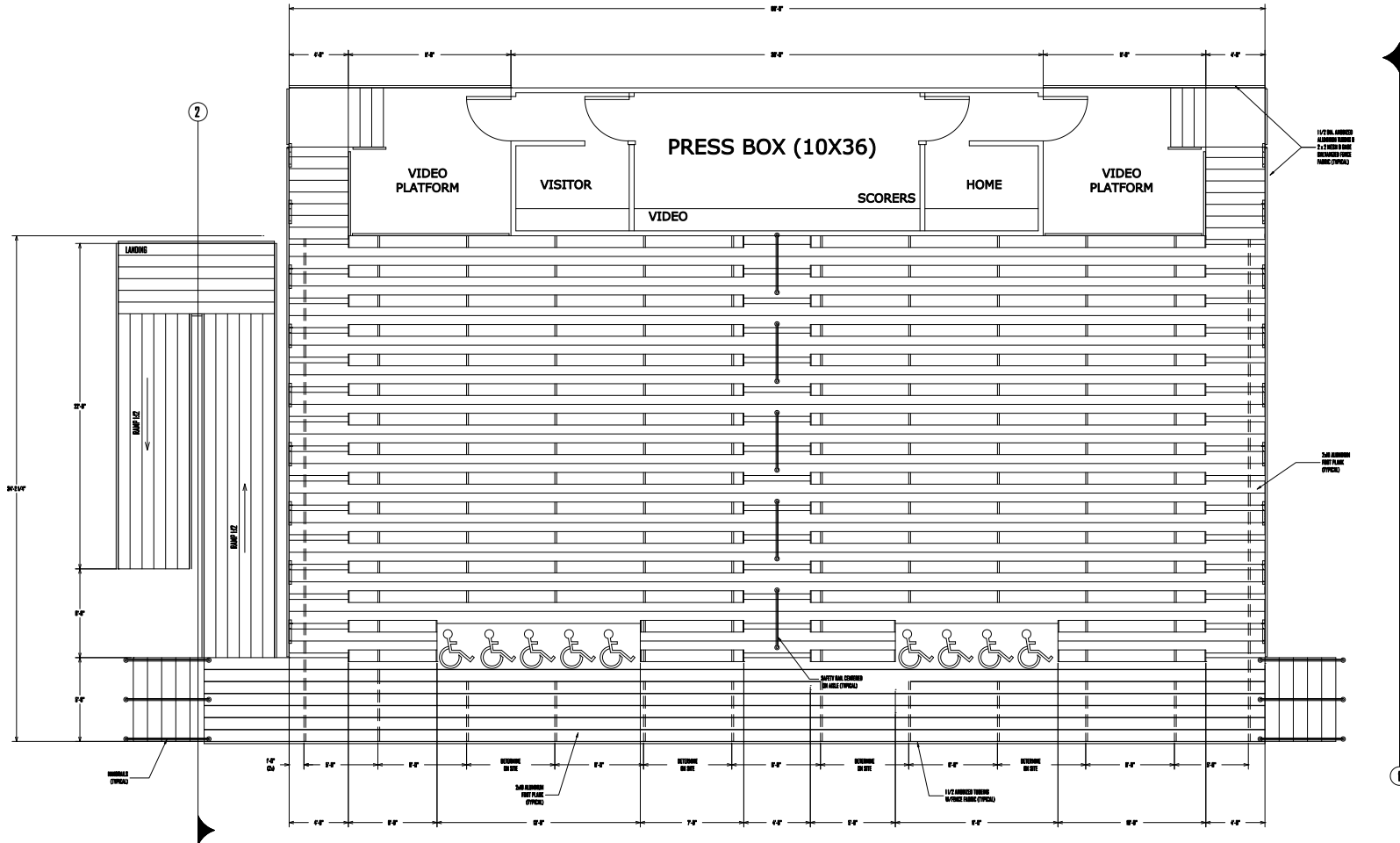
STADIUM HOME-SIDE BLEACHERS TOP PLAN
