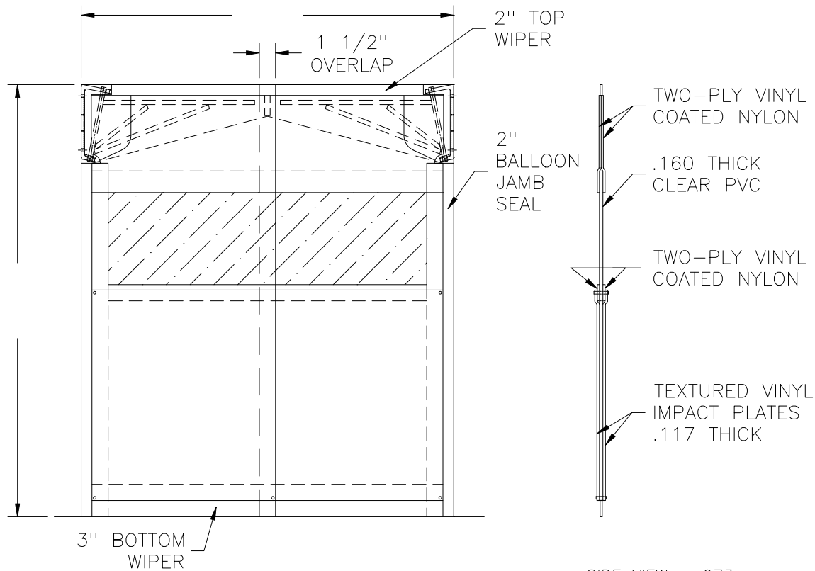
SIDE VIEW - 973
