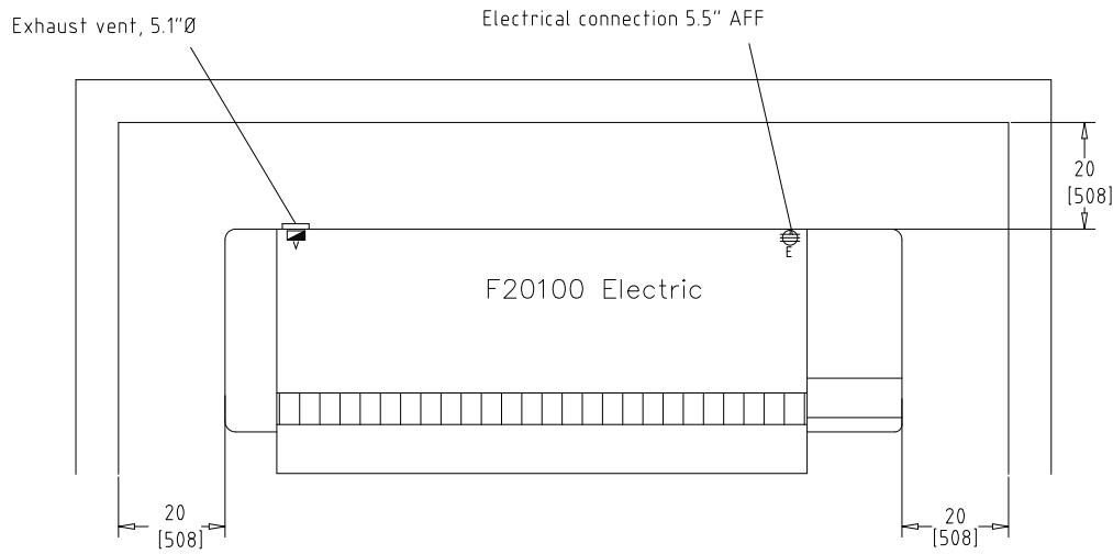
This symbol can be used for ironer model F20100 electric
