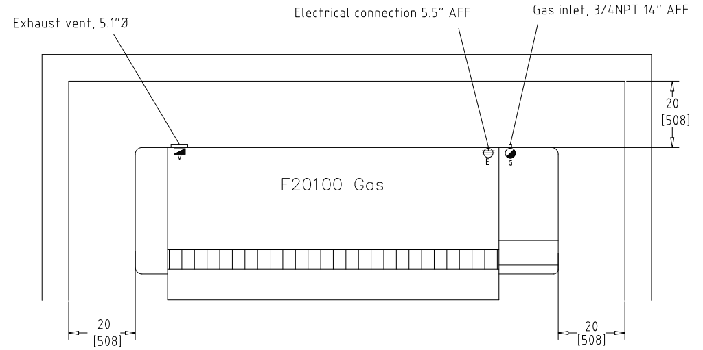
This symbol can be used for ironer model F20100 gas
