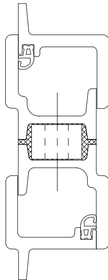
OPEN OUT
