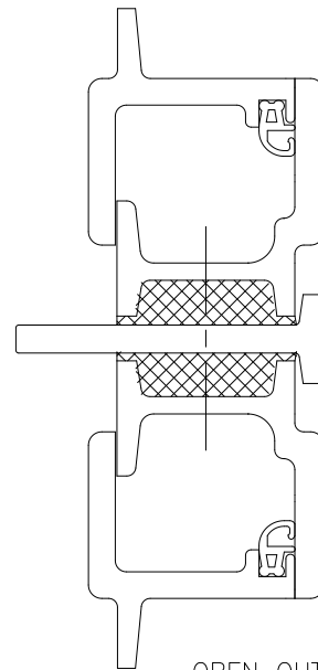
OPEN OUT
