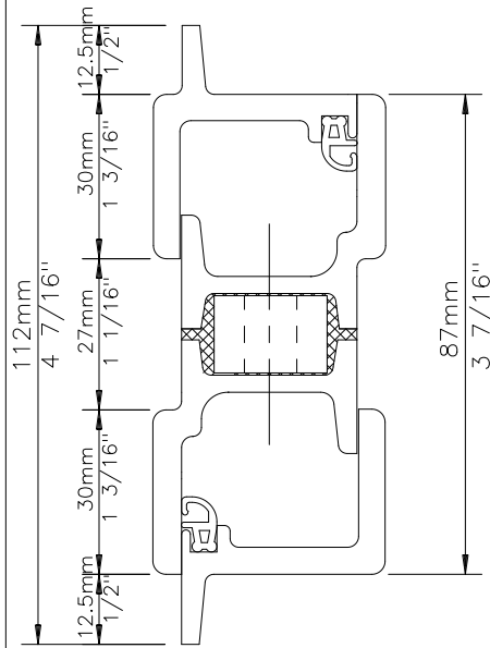
OPEN IN
