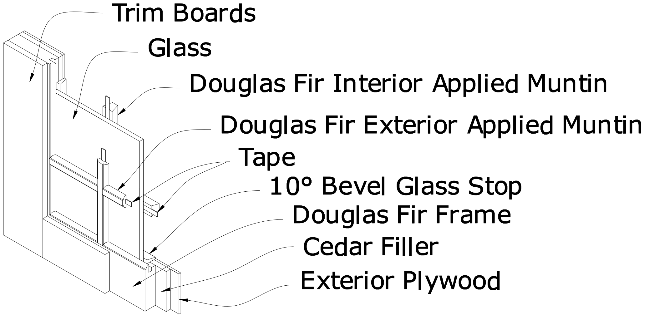
Standard Window Section Construction (Simulated Divided Lites Shown)
