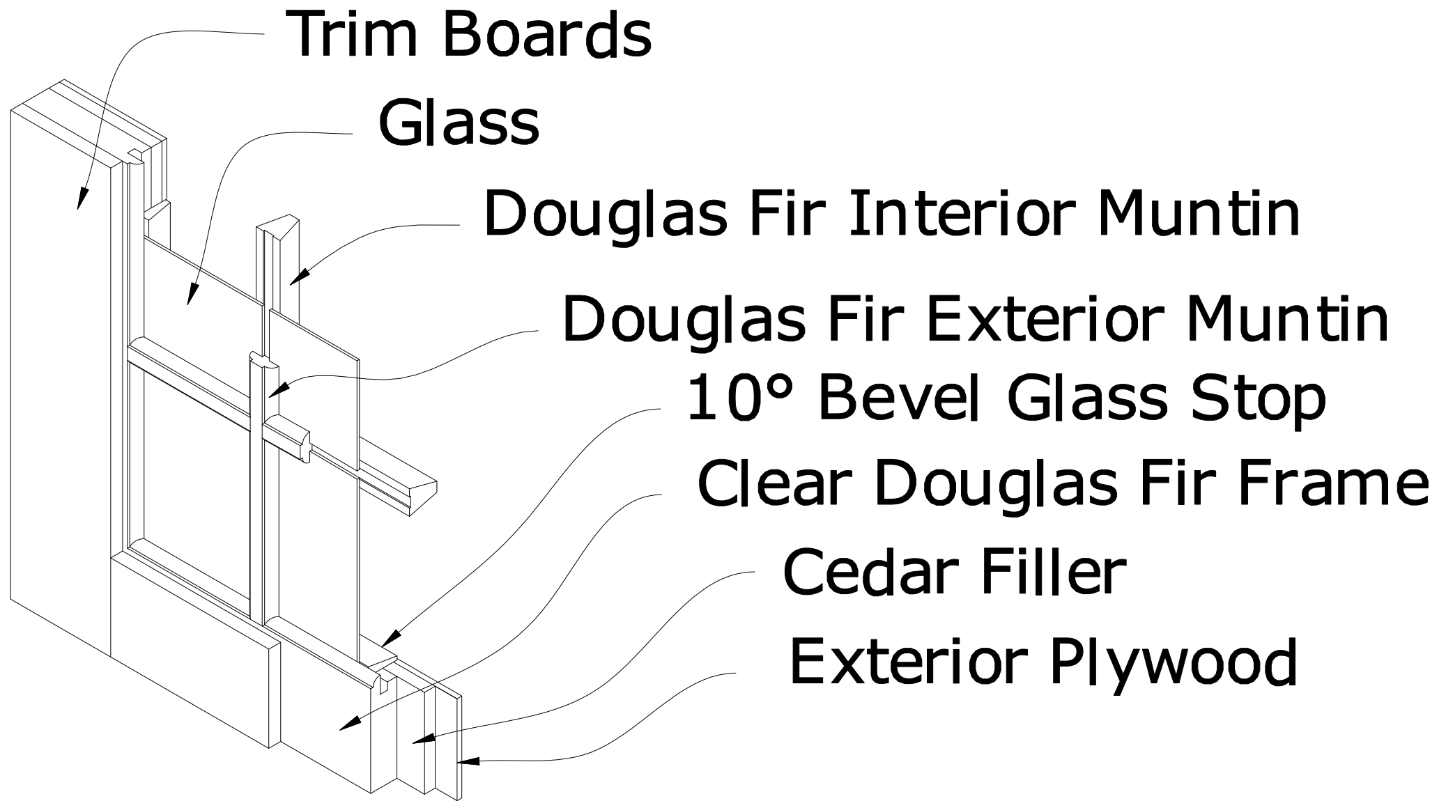
Standard Window Section Construction (True Divided Lites Shown)
