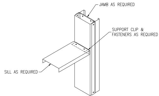
SILL DETAIL
