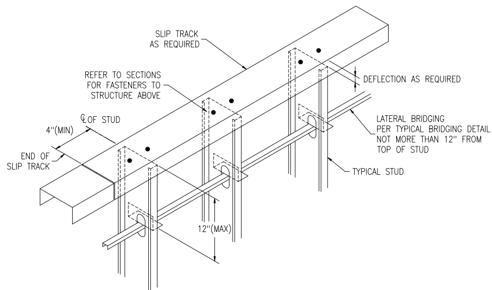
SLIP TRACK DETAIL
