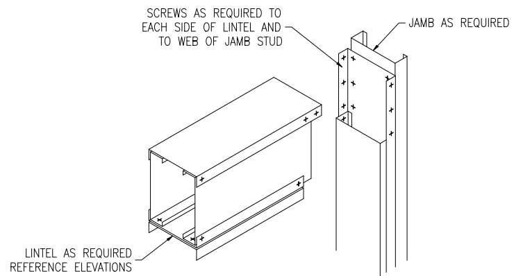
LINTEL DETAIL
