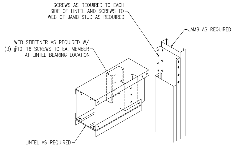
LINTEL DETAIL
