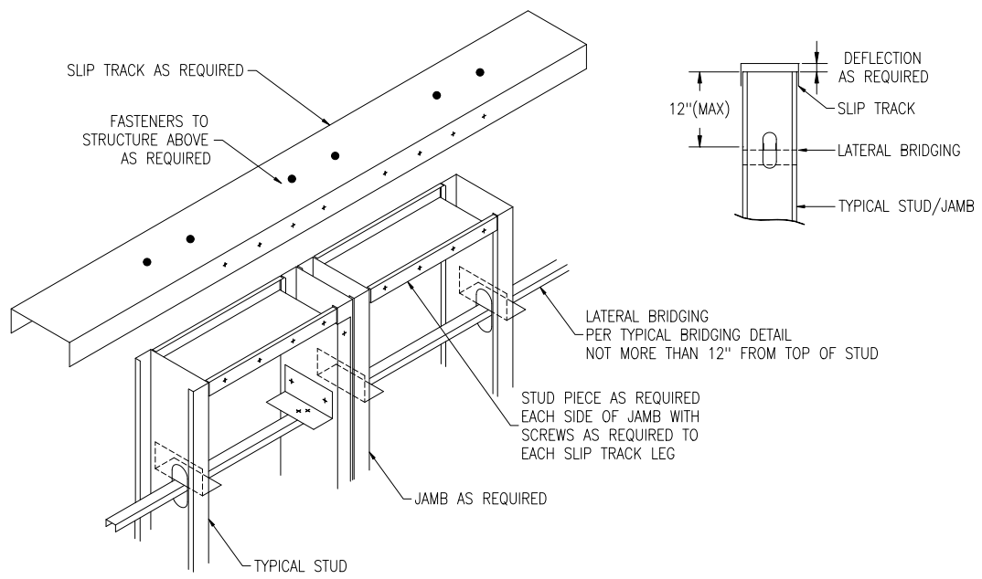
SLIP TRACK DETAIL
