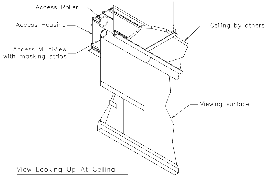
Mounting Detail
