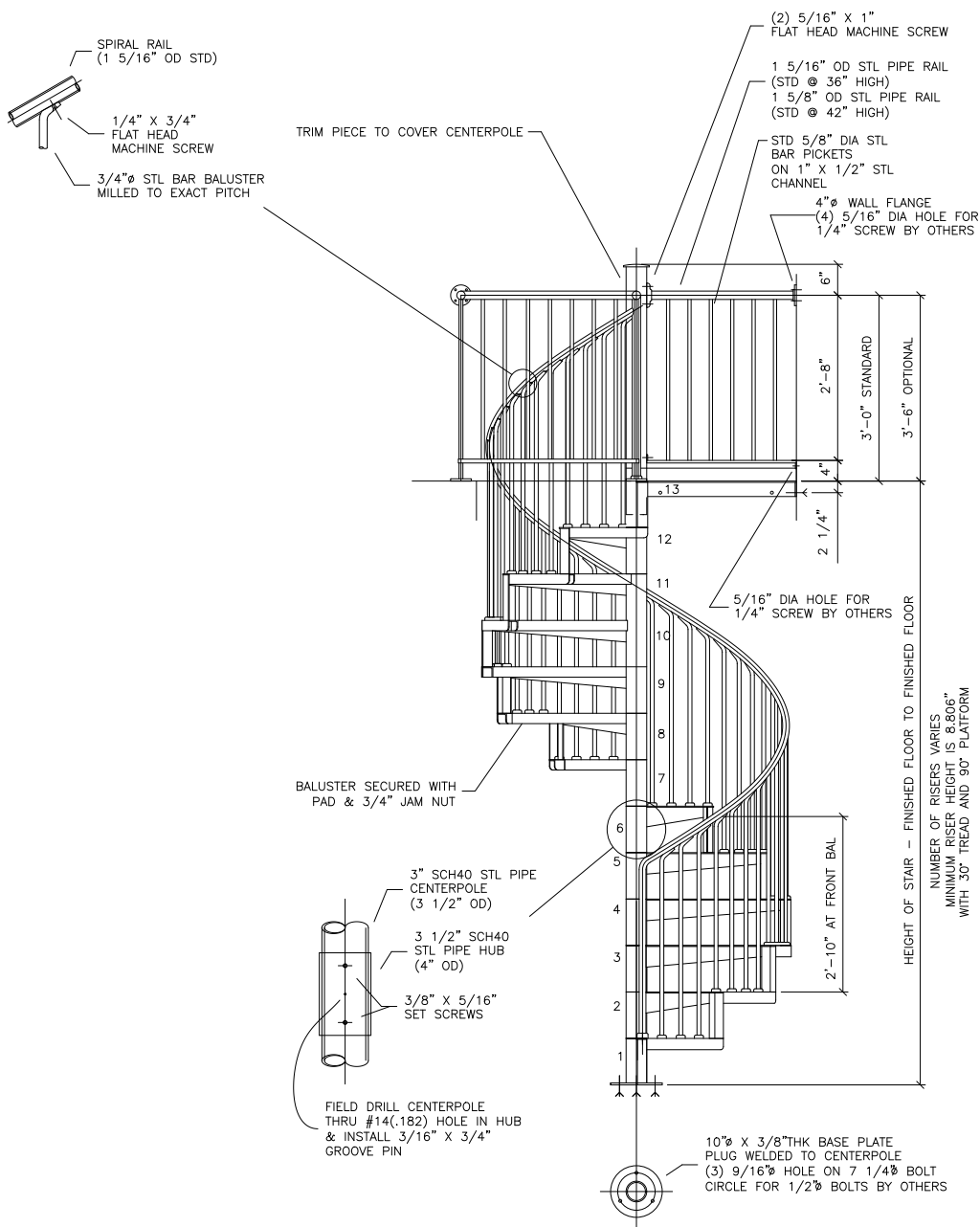
TYPICAL ELEVATION
