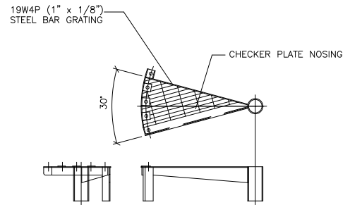
TYPICAL TREAD
