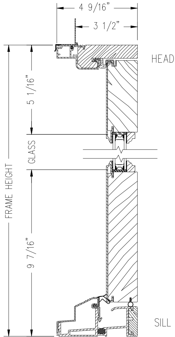
VERTICAL SECTION
