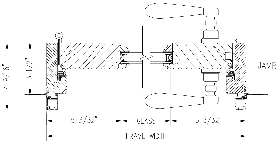
HORIZONTAL SECTION
