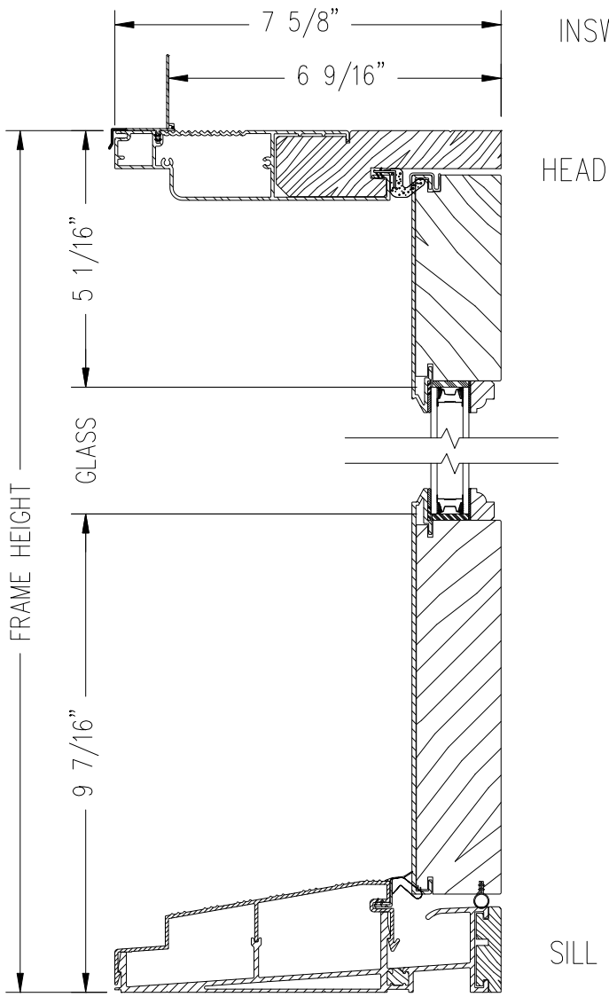
VERTICAL SECTION
