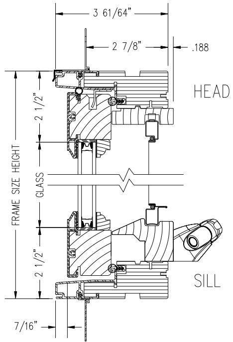
VERTICAL SECTION
