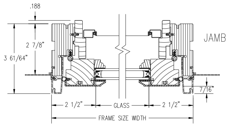
HORIZONTAL SECTION
