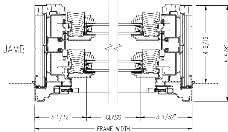
HORIZONTAL SECTION
