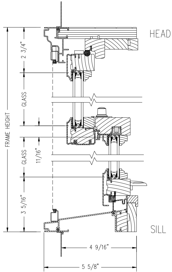
VERTICAL SECTION
