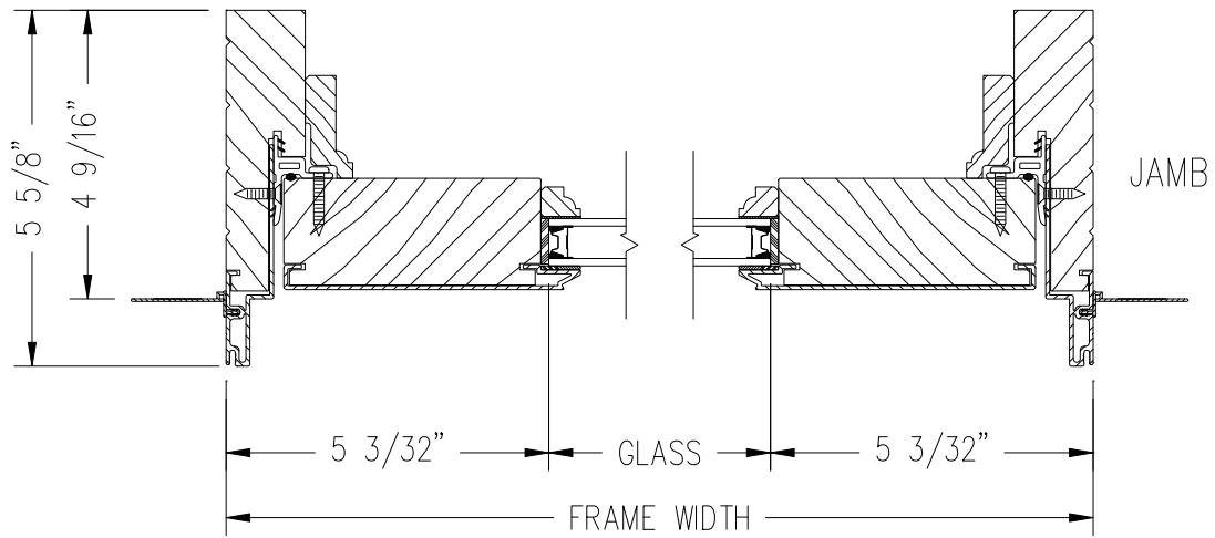
HORIZONTAL SECTION
