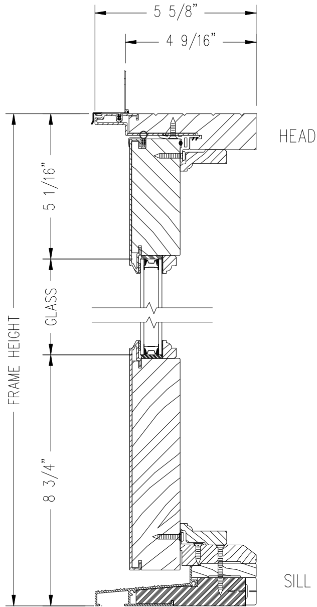
VERTICAL SECTION
