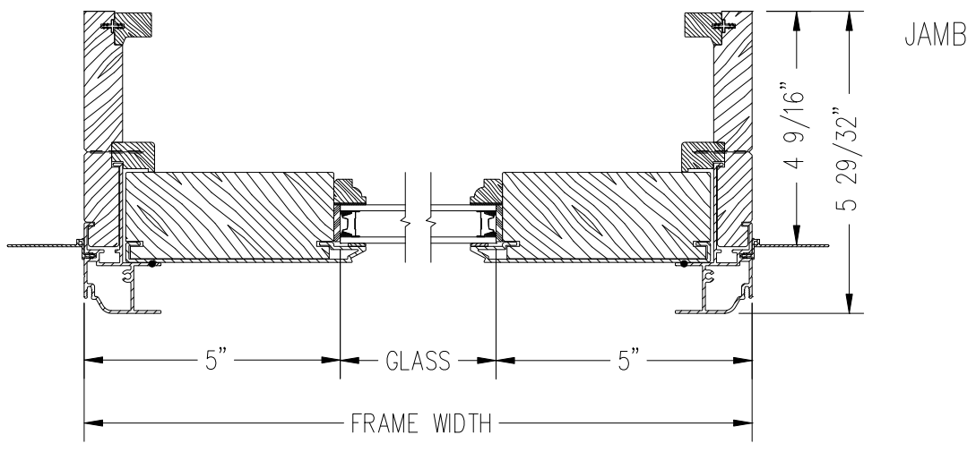
HORIZONTAL SECTION
