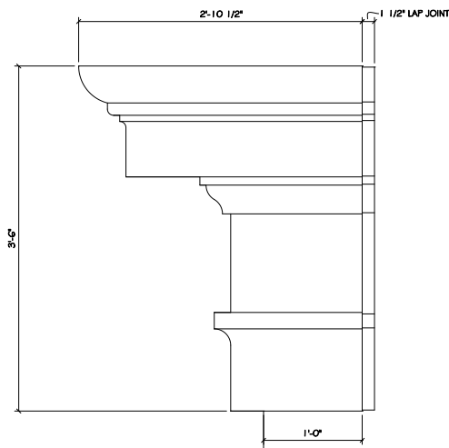
5 ELEV. OF OUTSIDE CORNER 4 SCALE: 1 1/2" = 1'-0"
