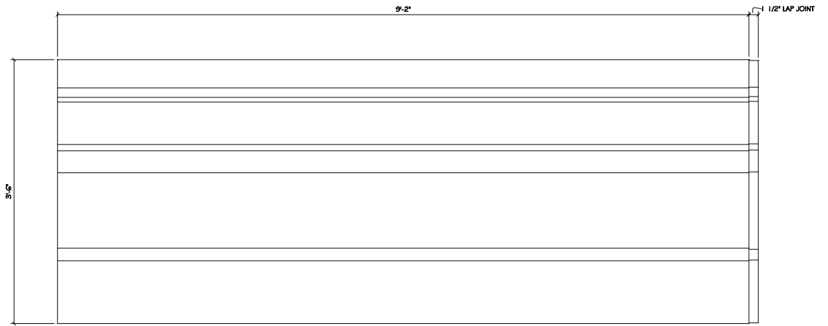
2 ELEVATION OF CR-150 4 SCALE: 1 1/2" = 1'-0"
