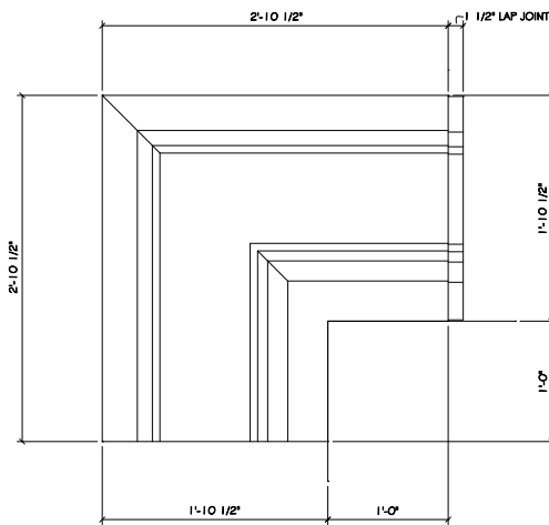
3 OUT. CORNER FROM BELOW 4 SCALE: 1 1/2" = 1'-0"
