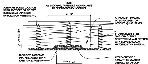
A LAP JOINT DETAIL 4 FULL SCALE
