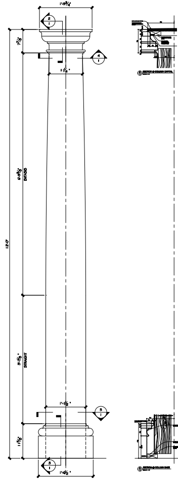
① ① ELEVATION OF EC-120F COLUMN COVER SCALE: 1/4" = 1'-0"
