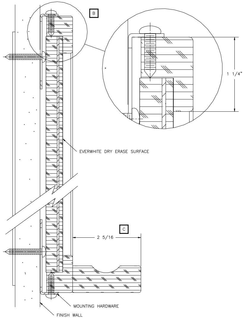
VERTICAL SECTIONS
