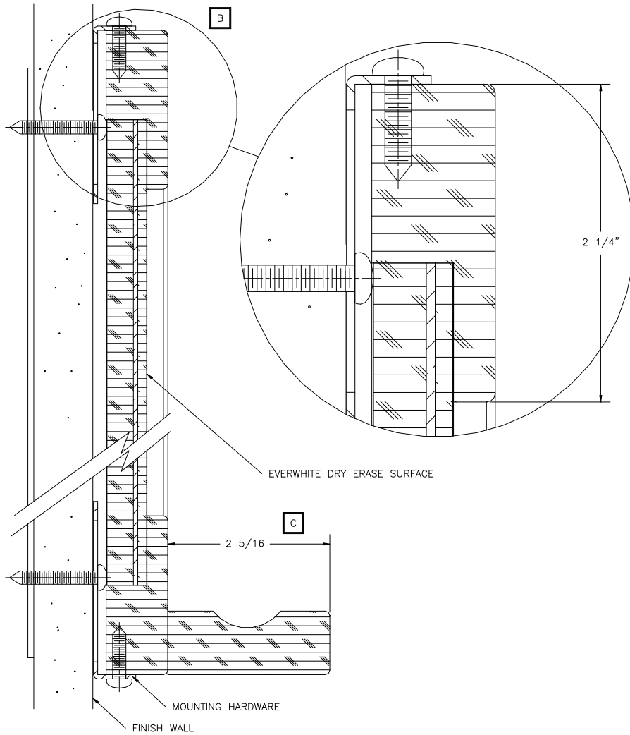
VERTICAL SECTIONS
